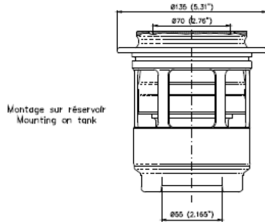
Female Coupling
